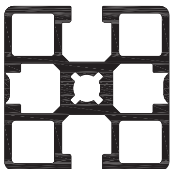
45 x 45 2GG 20.1099/0
