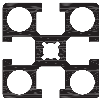
45 X 45 20.1006/0
